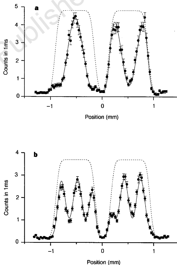
Figure 2 Spatial fringe pattern in the far field of the interferometer. The data were obtained with t_{\text{Bragg}} = 45\ \mu\text{s} , and the 50% beam splitter was realized with |U_0| = \hbar\pi t_{\text{Bragg}} . We chose t_{\text{sep}} = 105\ \mu\text{s} with d = 1.3\ \mu\text{m} (a), and t_{\text{sep}} = 255\ \mu\text{s} with d = 3.1\ \mu\text{m} (b). In both cases, the fringe period is in good agreement with the theoretical expectation. Each solid line represents a fit to the experimental data. The best-fit values for the visibilities are (75 \pm 1)\% and (44 \pm 1)\% , respectively. The reduced visibility for the case of the narrow fringes is due to the finite position resolution of our apparatus. The dashed lines represent the independently measured beam envelope, which consists of two broad peaks. The right peak is due to beams F and G (see Fig. 1), with a shape determined by the momentum distribution of the initial beam A. The left peak is a combination of beams D and E. It is a Bragg-reflected picture of the right peak. The fringe patterns under these two broad peaks are complementary, that is, the interference maxima in the left peak correspond to interference minima in the right peak, and vice versa.
