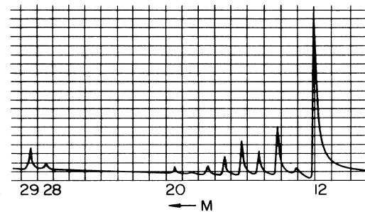
FIG. 11. First mass spectrum achieved with the ion trap. Gas: air at 2 \times 10^{-9} Torr (Rettinghaus, 1967).
