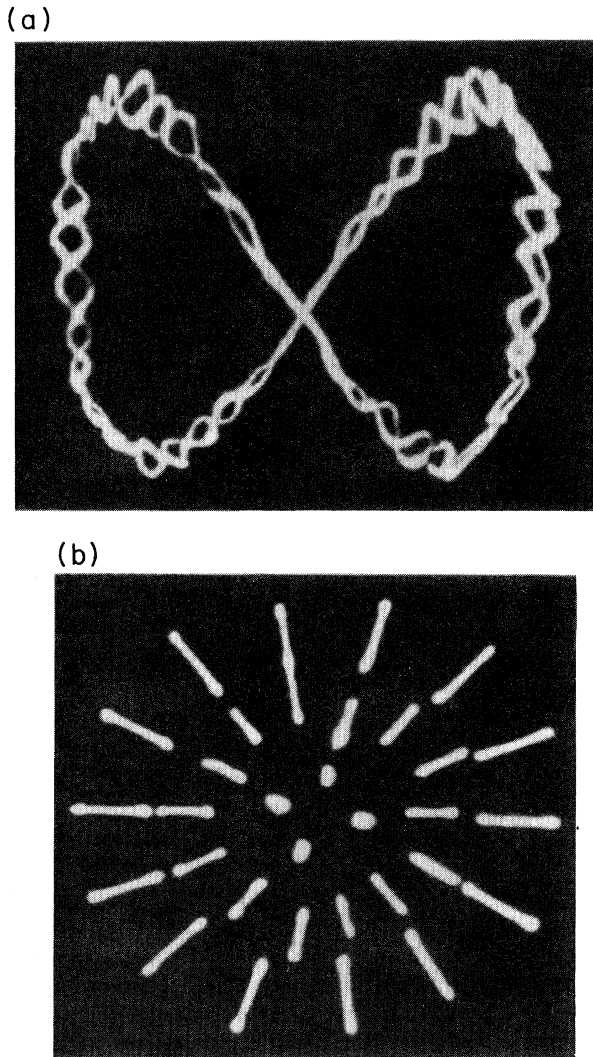
FIG. 9. (a) Photomicrograph of a Lissajous orbit in the r - z plane of a single charged particle of aluminum powder. The micromotion is visible. (b) Pattern of "condensed" Al particles (Wuerker and Langmuir, 1959).
