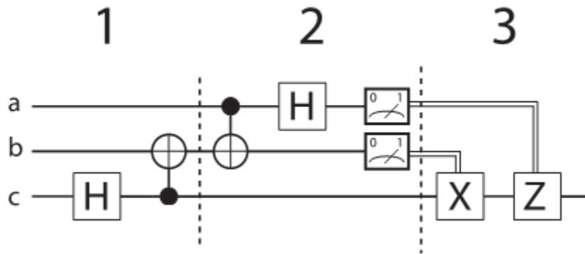
FIGURE 1.6.1. Teleportation Protocol Circuit Diagram. Part 1 creates the entanglement of the messenger qubit, b , with the receiver qubit c . Part 2 is the interaction of the messenger qubit and the transmission qubit, a , and full state measurements of the two qubits afterward. Part 3 is the classical transfer of information about the measured state of qubits a and b with the conditional Pauli gates to act on qubit c if the corresponding qubit was found in the excited state.
